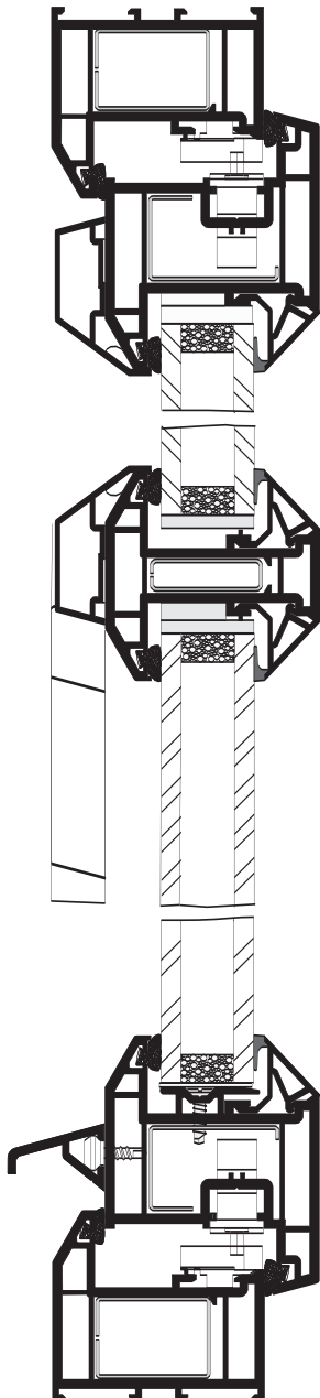
Cross Section through the Mock Sash
