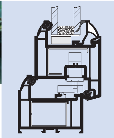
Large outerframe with tilt and turn sash
